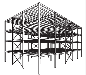
Illustration 17: construction à poteaux-poutres
